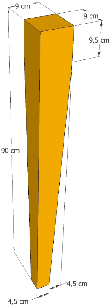
ISOMETRIC VIEW
