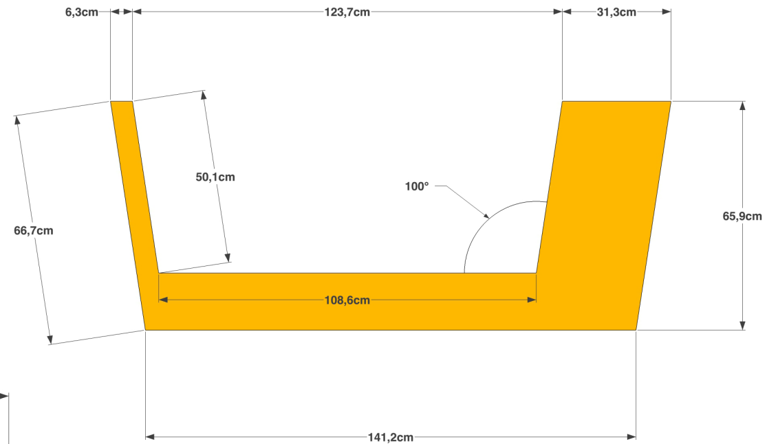
PART 1 DETAIL
