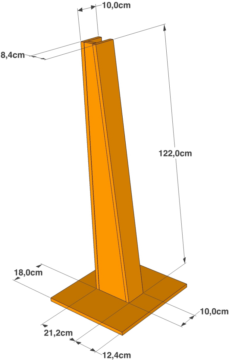
STAND DETAIL FRONT VIEW
