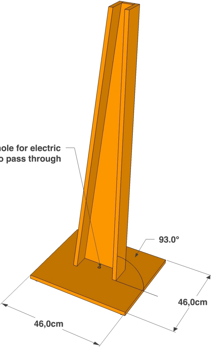
STAND DETAIL BACK VIEW
